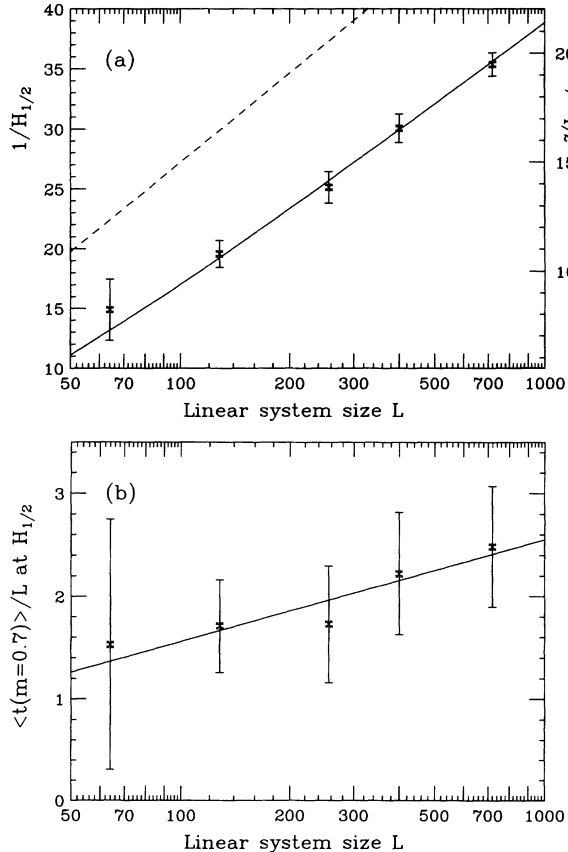
FIG. 5. Inverse field and mean lifetime at the DSP. (a) The estimates 1/H_{1/2} for 1/H_{\text{DSP}} as obtained from Fig. 4, shown vs L on a logarithmic scale. The solid curve corresponds to L\alpha R_0 with b+c=2 in Eq. (10b) and with the proportionality constant adjusted to minimize the weighted sum of squares. The dashed line indicates the asymptotic slope 3/\Xi(0.8T_c) . (b) The average lifetimes at 1/H_{1/2} . The solid straight line is a weighted least-squares fit. The figure supports the asymptotic behavior given in Eq. (18), \langle t \text{ at } H_{\text{DSP}} \rangle \propto L \ln L . See details in Sec. IV.
