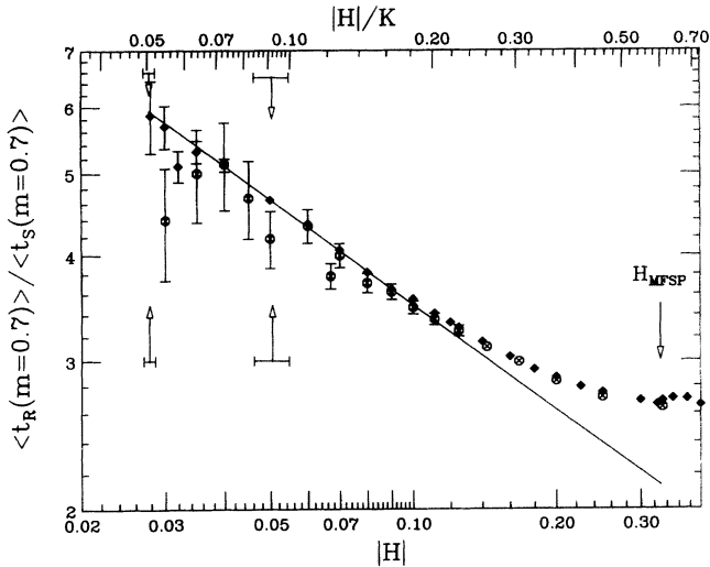
FIG. 7. The ratio \langle t_R \rangle / \langle t_S \rangle between the mean lifetimes obtained with random and sequential MC updates for L=128 and 720. The symbols and parameters are the same as in Figs. 3 and 8. The two pairs of opposing arrows with horizontal error-bar “feathers” mark H_{1/2} for the two system sizes. The solid straight line in this log-log plot is a weighted least-squares fit to Eq. (22) in the weak-field part of the multidroplet region for L=720 . See details in Sec. IV.
